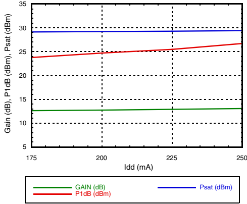
Gain & Power vs. Supply Current @ 16 GHz
